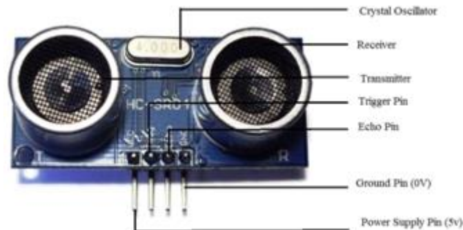
Figure 3.2: Basic working principle of the Ultrasonic Sensor
